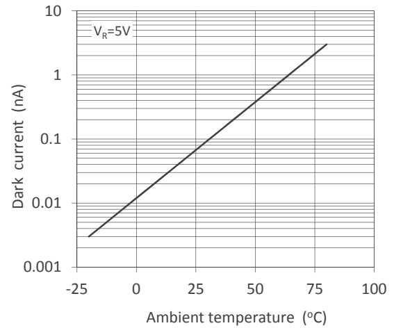
Dark Current - Ambient Temperature
